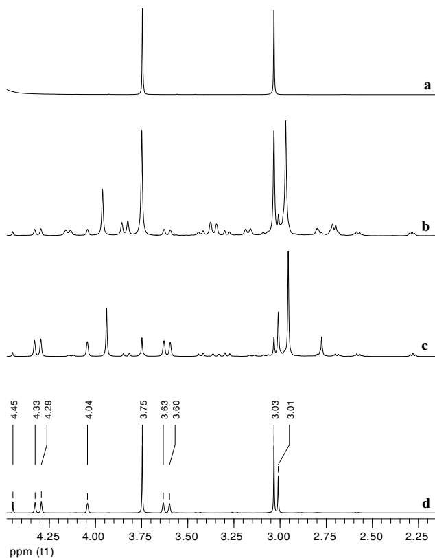
Fig. 1. ^1\text{H} NMR spectra of a reaction mixture of 2 (1.41 M) and \text{NH}_4\text{F} (4.50 M) in a \text{D}_2\text{O} at (a) t = 0 s, (b) t = 20 min 17 s, and (c) t = 440 min. (d) ^1\text{H} NMR spectrum of a mixture of 1 (0.09 M), 2 (0.09 M), and 3 (0.01 M) in \text{D}_2\text{O} .
