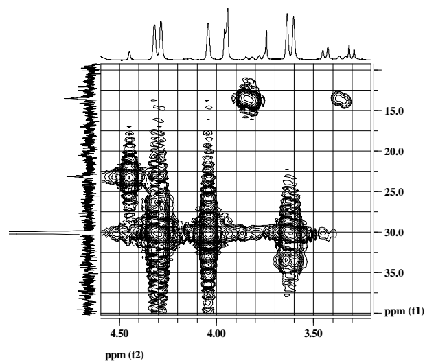
Fig. 5. 1 H– 15 N HMBC contour plot of reaction mixture.
