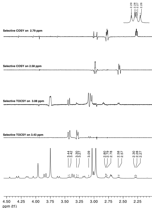
Fig. 3. 1 H NMR-selective irradiation experiments for 7 .
