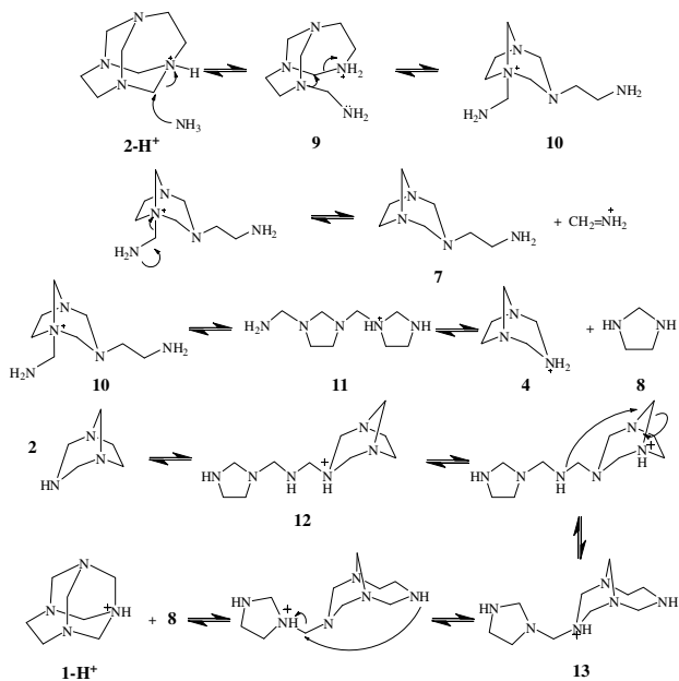
Scheme 1. Proposed mechanism for forming compound 1 .
