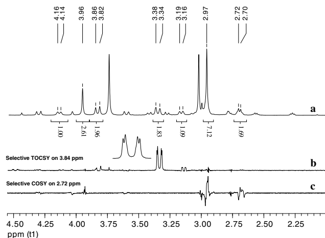
Fig. 2. TOCSY-selective experiments for 4 .
