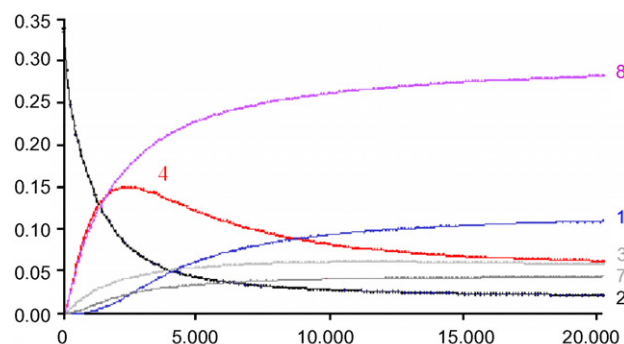
Fig. 4. Concentration (mM) versus time (s) for 1 , 2 , 3 , 4 , 7 , and 8 in the reaction of TATD with \text{NH}_4\text{F} .
